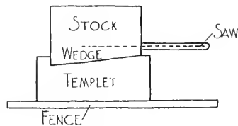
FIG. 169. SAWING WEDGES.
